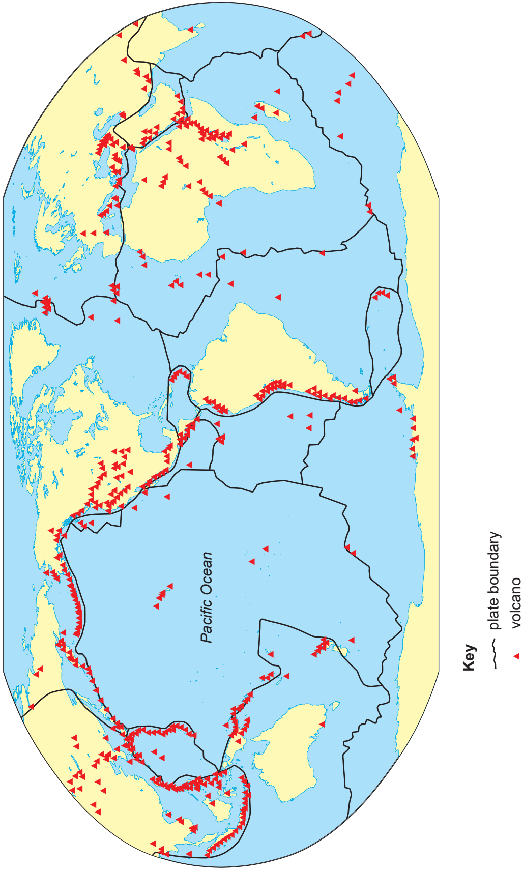
Fig. 4.1 for Question 4 The global distribution of volcanoes
